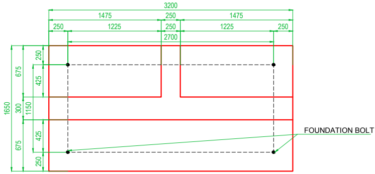
PLAN
